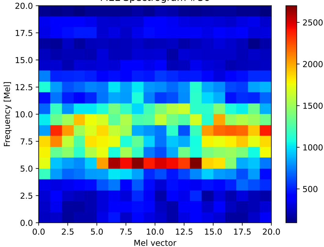
MEL Spectrogram #36
